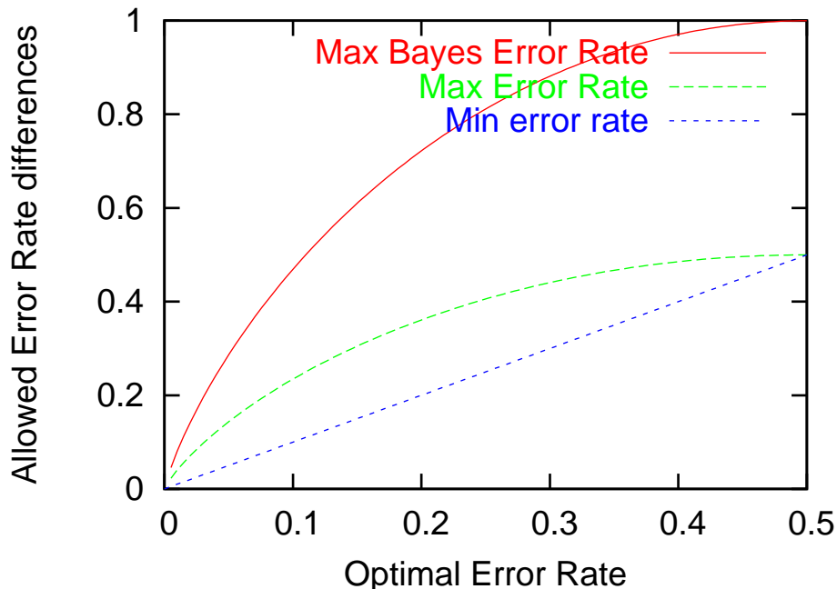
Fig. 1. A graph depicting the set of asymptotically allowed error rates for different classification algorithms. The x -axis depicts the optimal classifier's error rate \mu (also shown as the straight line). The lower curve is just 0.5H(\mu) and the upper curve is H(\mu) . Theorem 2 says that any (\mu, \mu') between the straight line and the lower curve can be achieved for some learning problem D and prior P . Theorem 3 shows that the Bayesian learner can never have asymptotic error rate \mu' above the upper curve.
