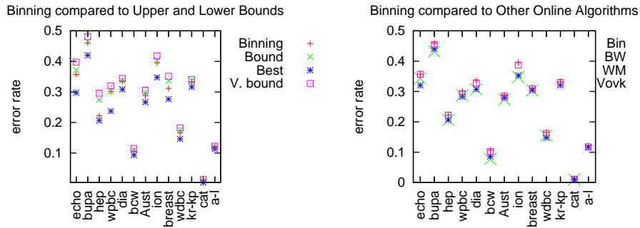
Fig. 1. In the table above we give the number of rounds, the number of experts, and the number of mistakes of the best expert. The datasets are ordered above by byte size. In the graph on the lower left we show how the performance of Binning compares to the upper Bound on Binning performance, the Best single expert, and the bound on Vovk’s algorithm. The right graph shows how the performance of Binning compares to Binomial Weighting (BW) (2 entries missing), Weighted Majority (WM), and Vovk’s algorithm.
